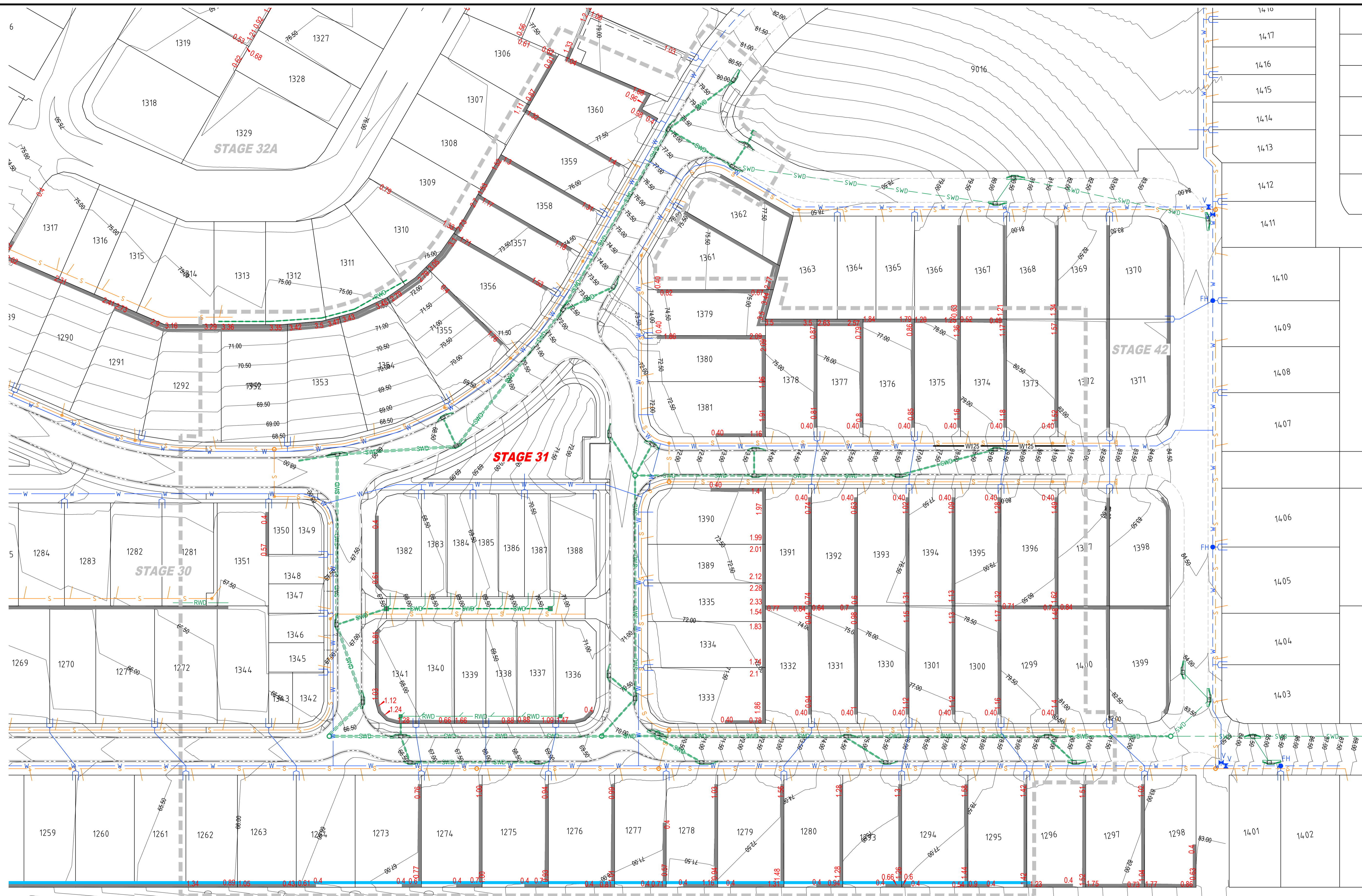
LAYOUT PLAN SCALE 1:500
